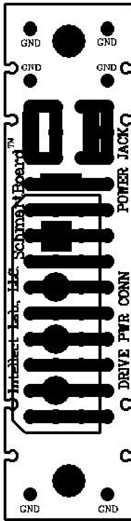
DRIVE POWER AND POWER JACK (201-0101-01)
