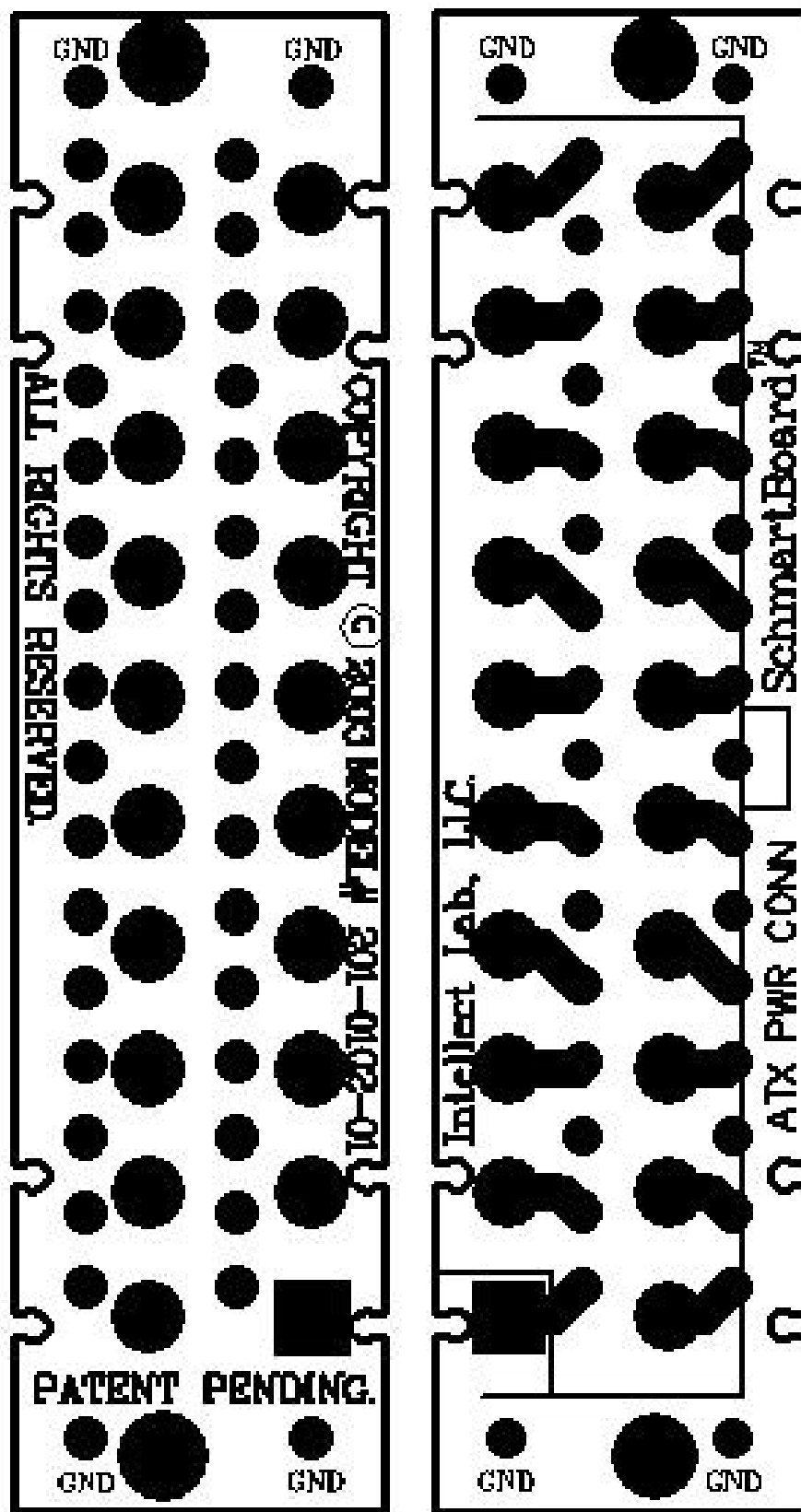
ATX POWER CONNECTOR (201-0102-01)
