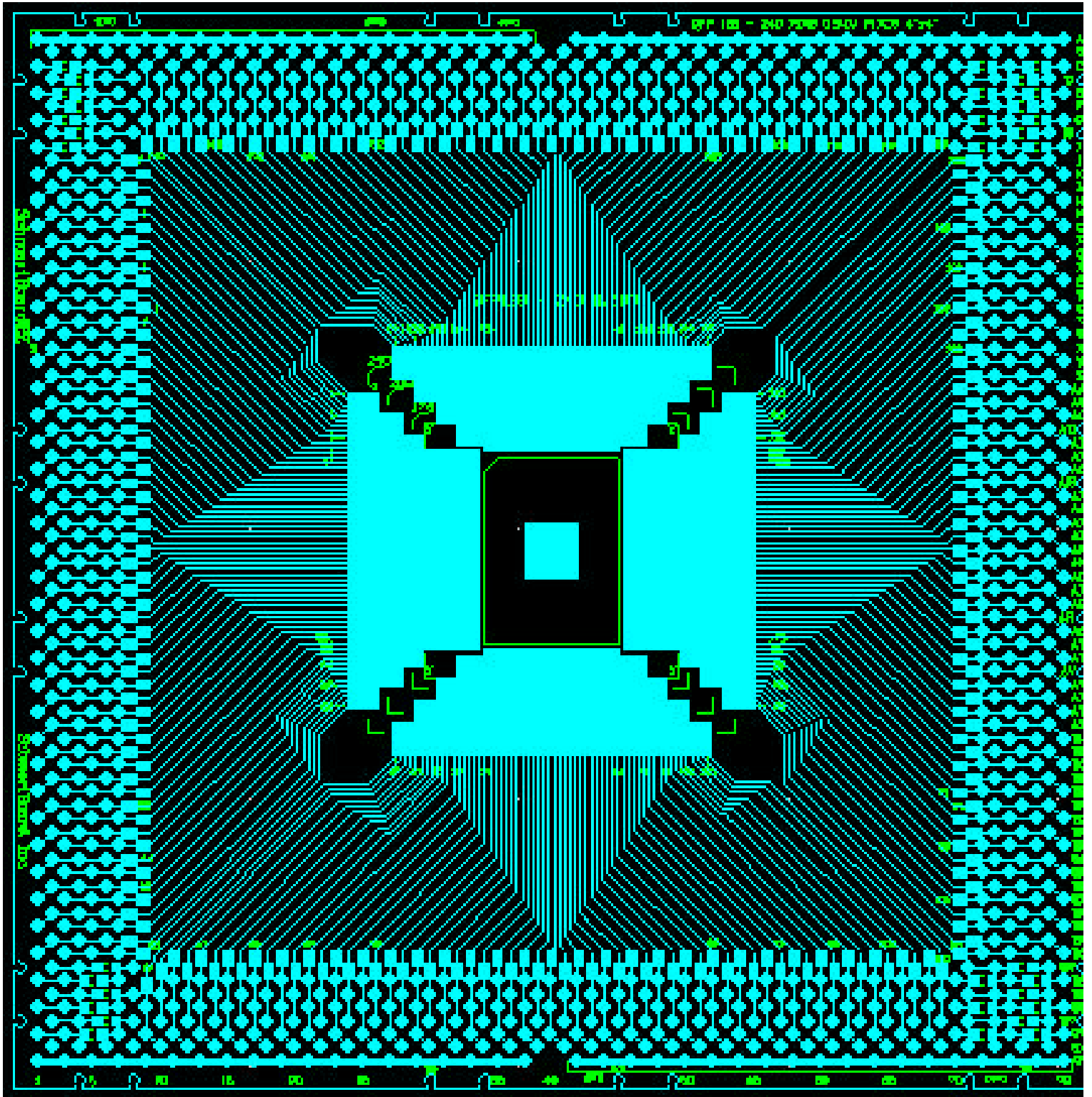
202-0032-01 SchmartBoard/EZ 4"x4" QFP 128-240 Pins 0.5mm Pitch
